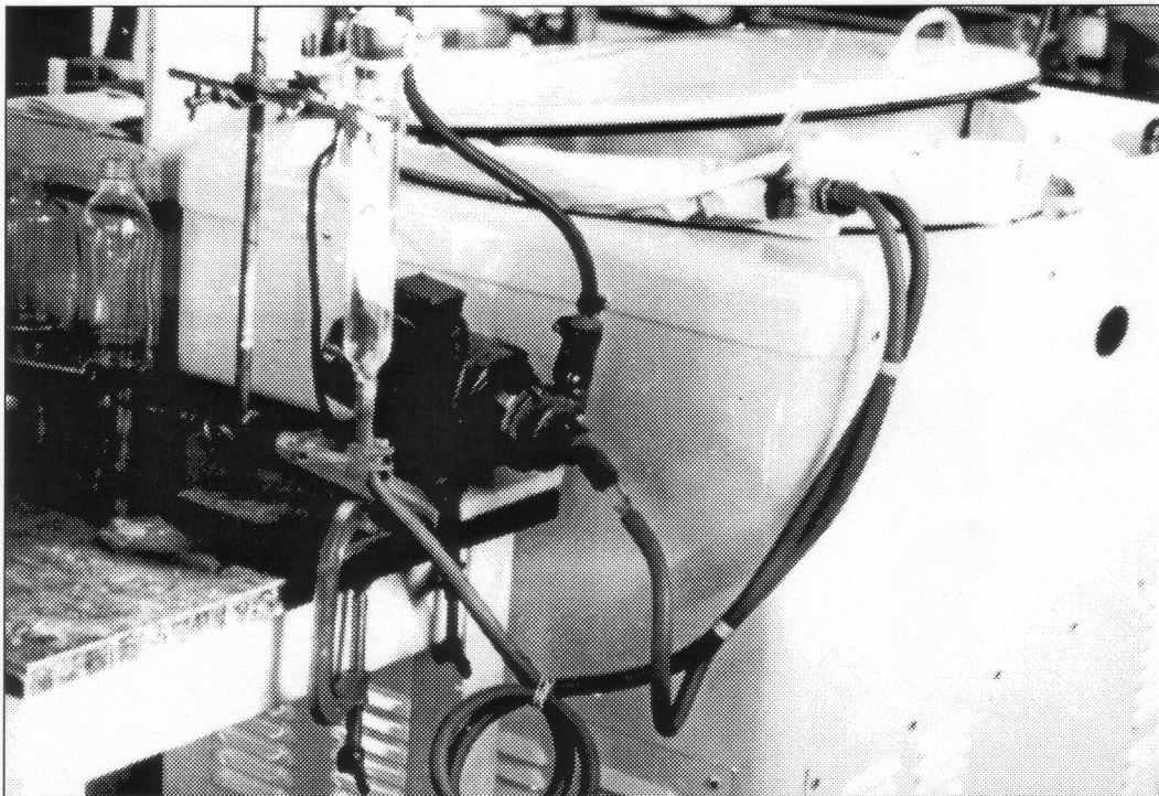
7. Most of the added salts must be removed by dialysis. Owing to the instability of material, this must be done rapidly. The apparatus is shown.
