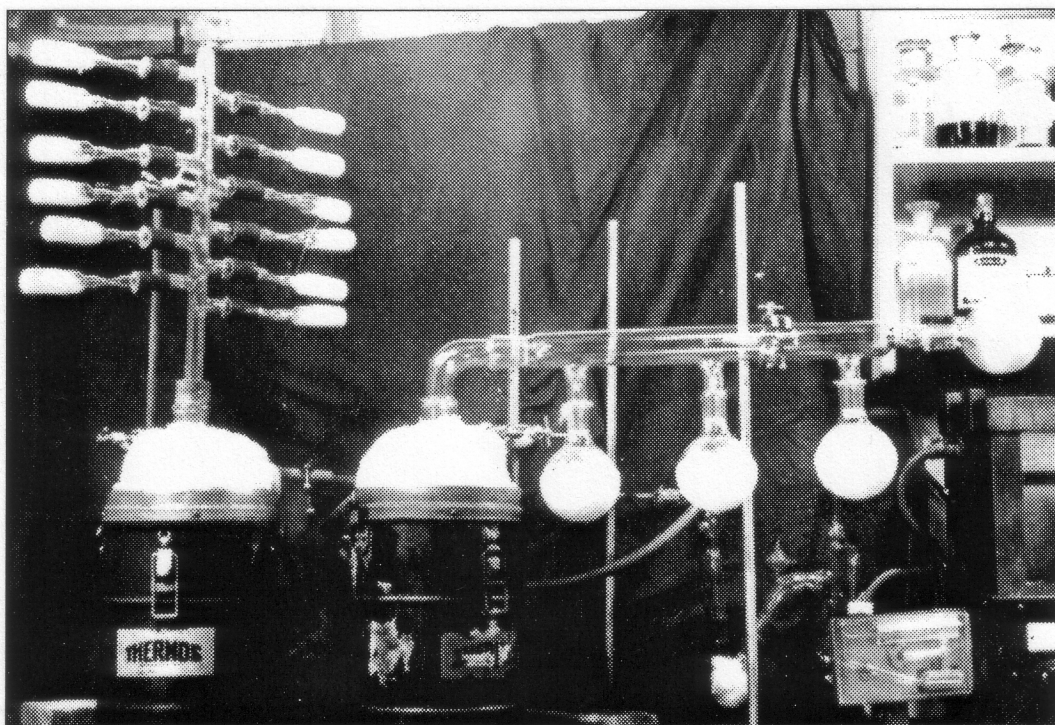
8. Preservation by freeze-drying.
